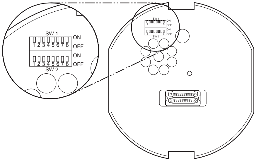
Figure 14. Switch Locations
